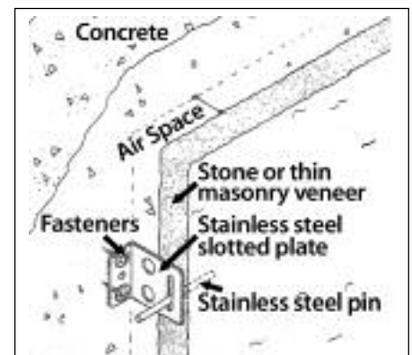
Figure 6 Slotted Heavy Duty Rap-Tie System Application for Dimension Cut Stone Veneer
