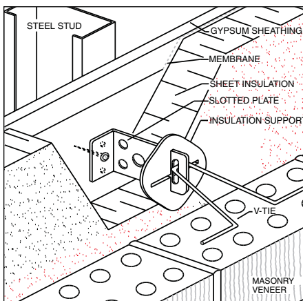
Figure 5 Slotted Heavy Duty Rap-Tie Surface Mounted on Protected Gypsum Sheathing
