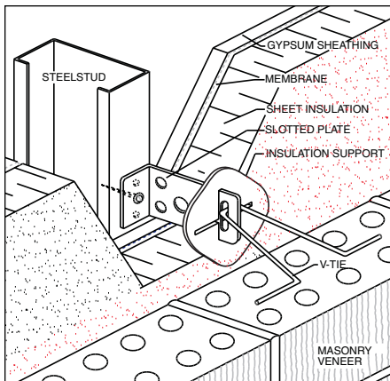
Figure 4 Slotted Heavy Duty Rap-Tie Attached Directly to Steel Stud
