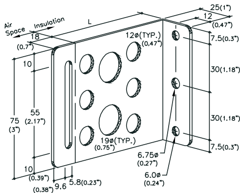
Figure 1 Slotted Heavy Duty L-Plate
