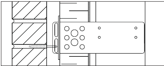
Figure 5 An installation wall section
