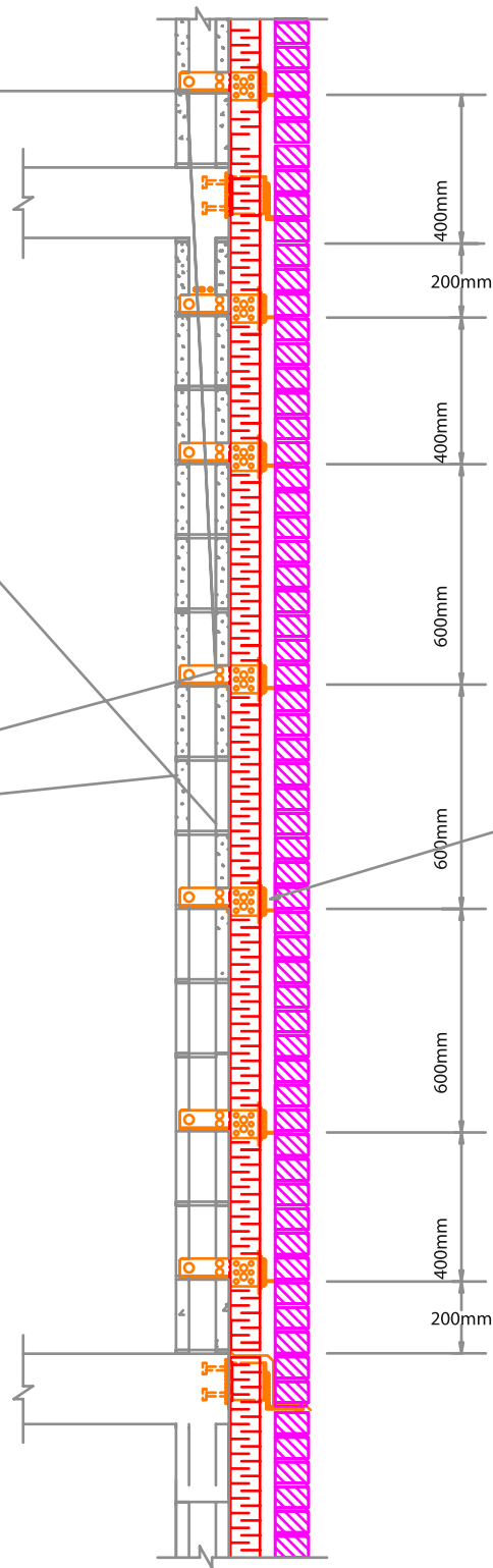
FIGURE 6 RECOMMENDED BLOCK SHEAR CONNECTORS SPACING FOR CONC. BLOCK-BRICK VENEER WALL
