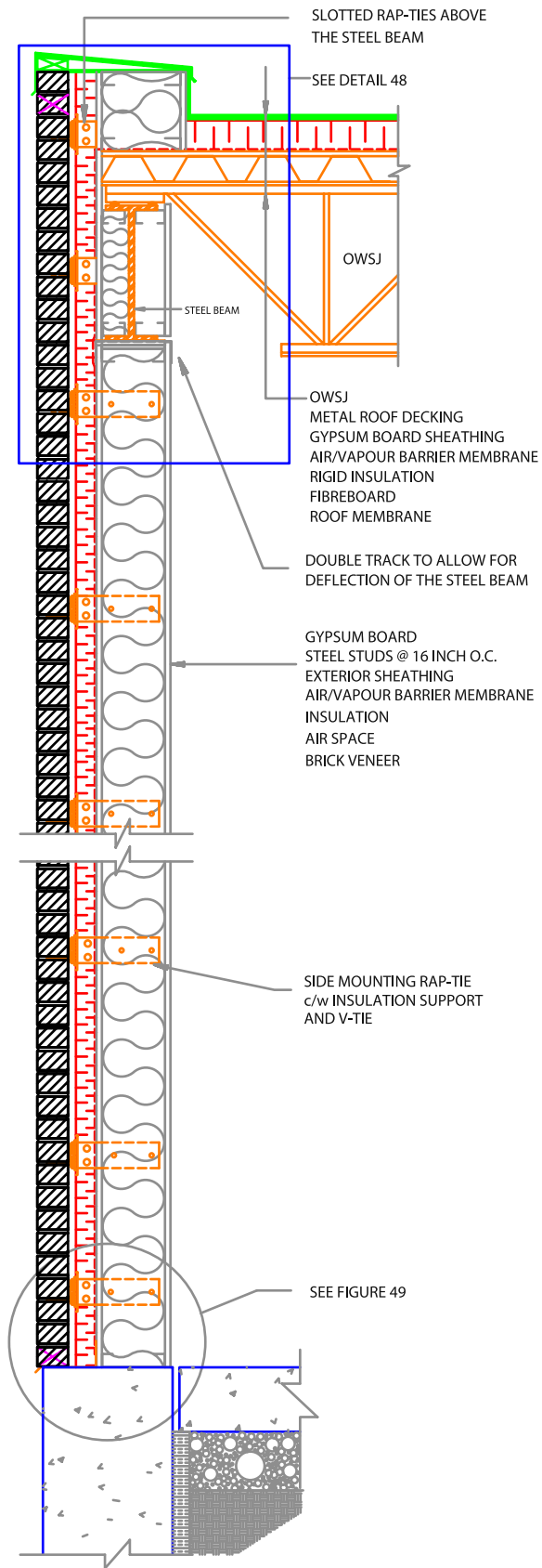
FIGURE 47 BRICK VENEER / STEEL STUD - O.W.S.J.
