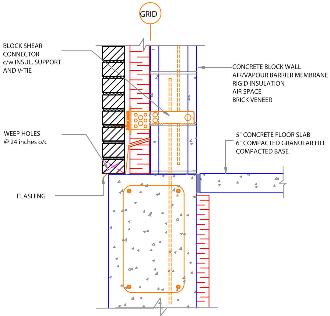
FIGURE 46 BRICK VENEER/CONCRETE BLOCK - AT FOUNDATION
