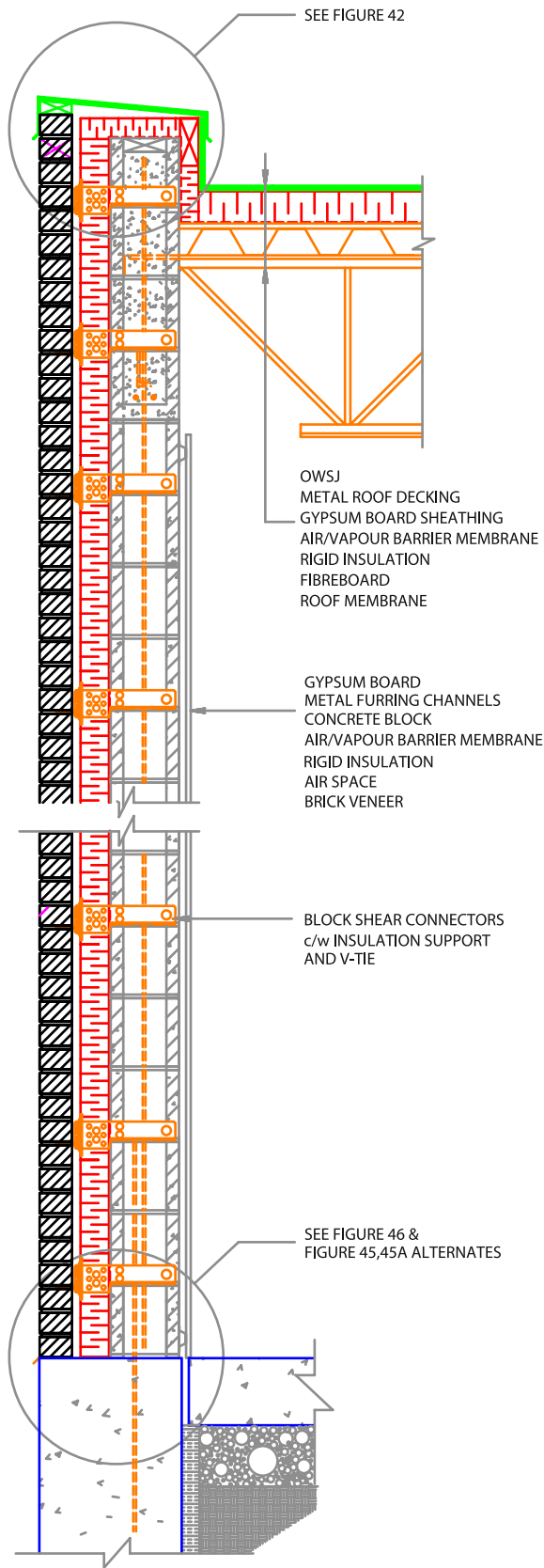
FIGURE 41 BRICK VENEER / CONCRETE BLOCK - O.W.S.J. CONNECTION NTS
