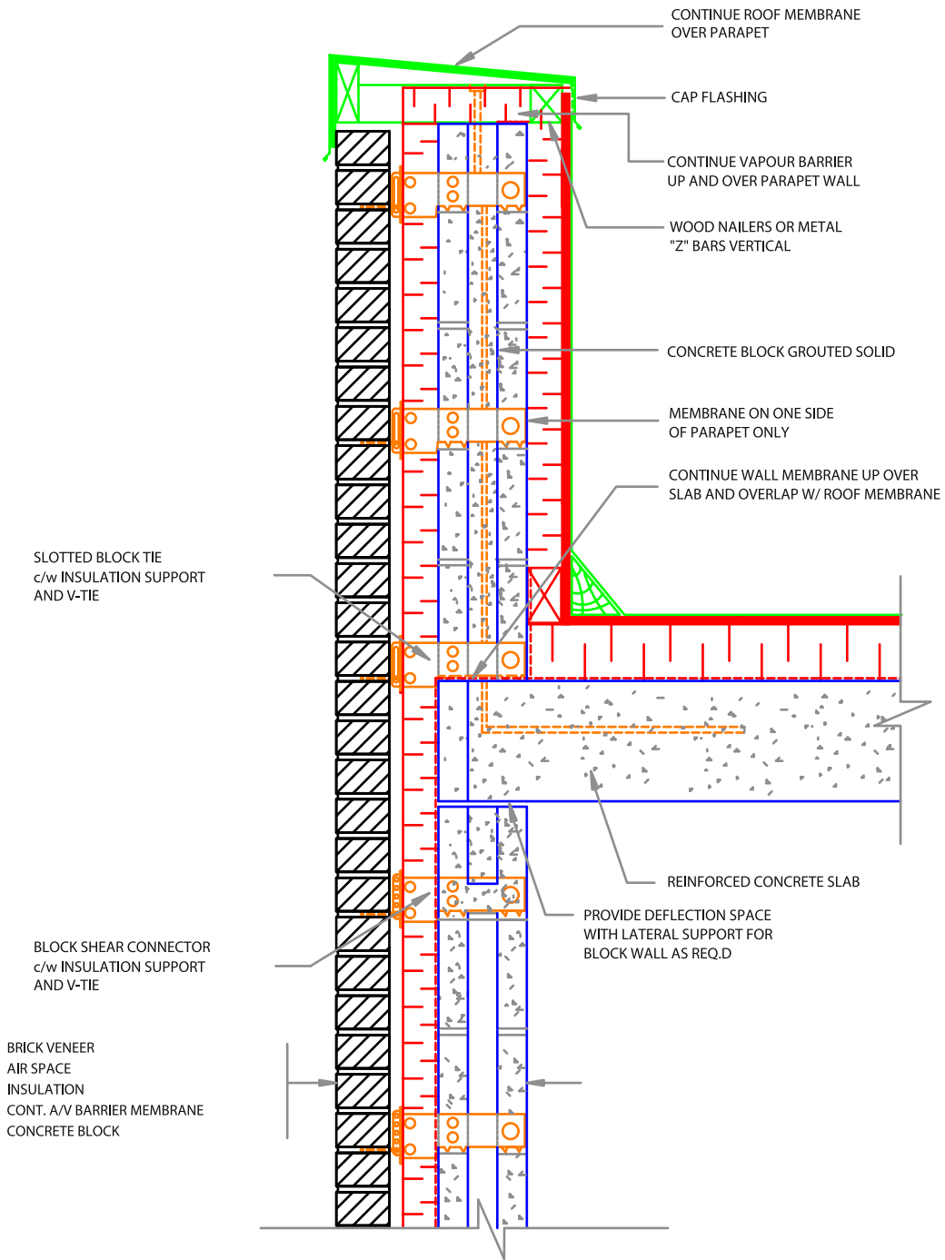
FIGURE 4 BRICK VENEER/CONCRETE BLOCK-DETAIL AT HIGH PARAPET FOR NON LOAD BEARING ASSEMBLY
