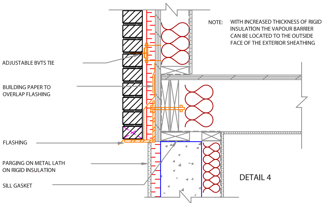
FIGURE 39 DETAILS OF BRICK VENEER AT GROUND AND FLOOR LEVELS (INSULATED CAVITY)
