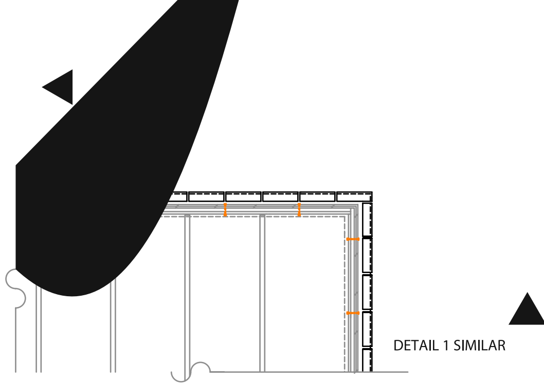
FIGURE 38 CORNER PLAN
