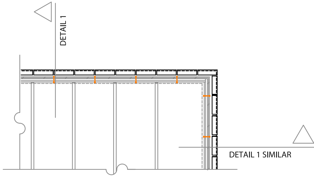
FIGURE 38 CORNER PLAN
