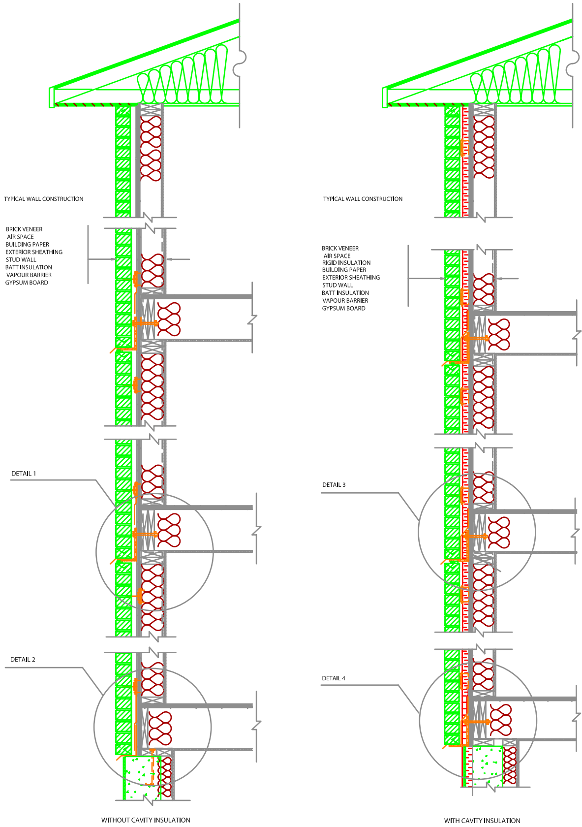
FIGURE 36 TYPICAL WOOD FRAME CONSTRUCTION APARTMENT BUILDING
