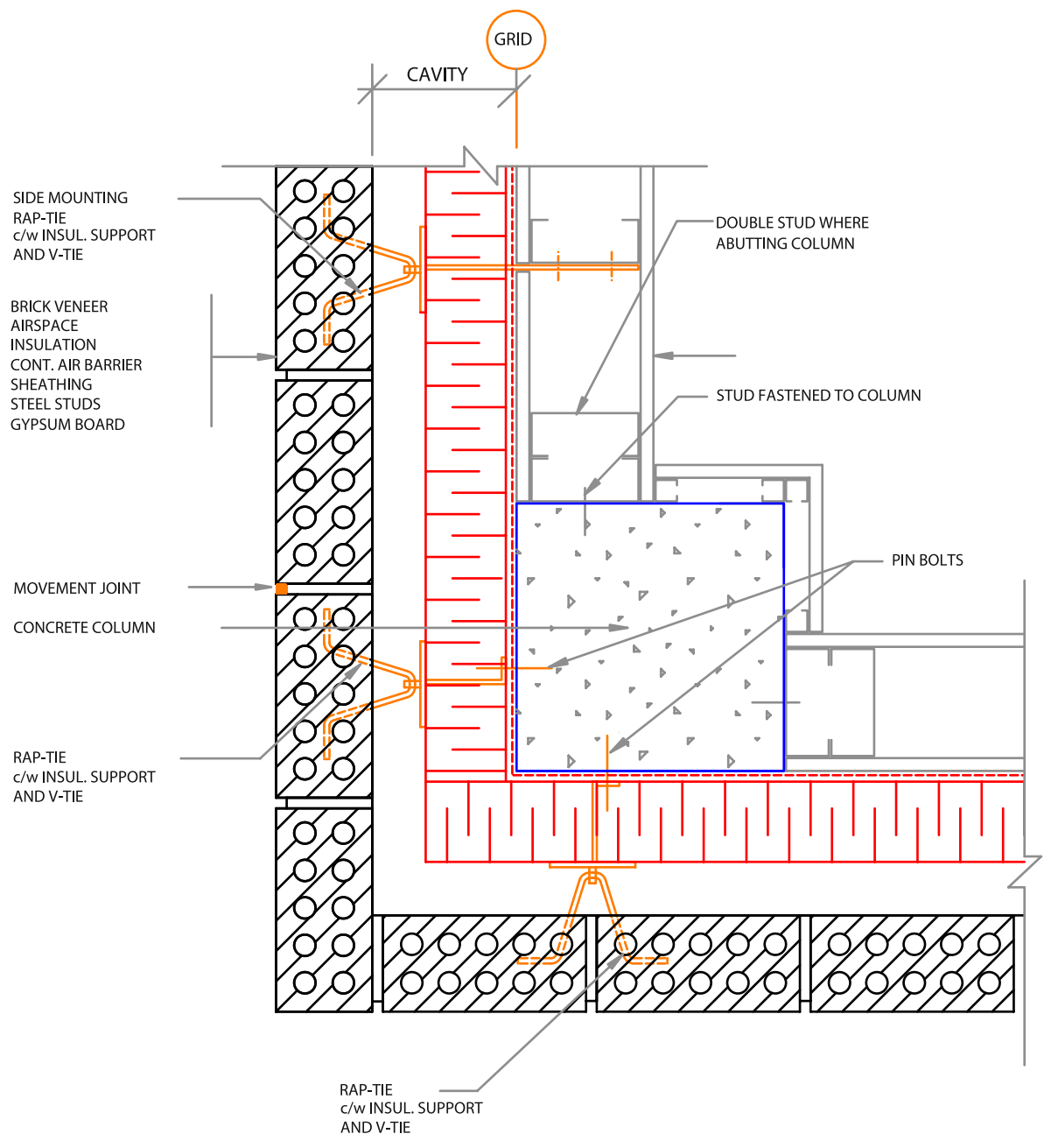
FIGURE 25 BRICK VENEER / STEEL STUD - CONTROL JOINT/AIR STOP
