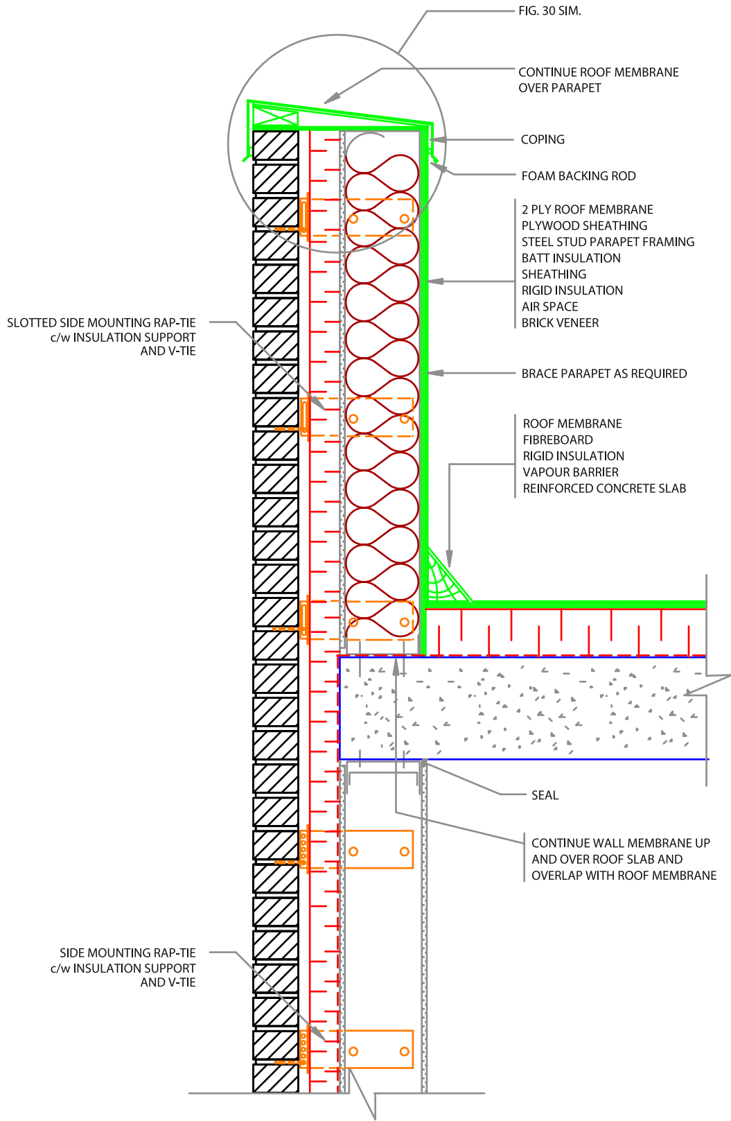
FIGURE 24 BRICK VENEER / CONCRETE BLOCK - DETAIL AT HIGH PARAPET
