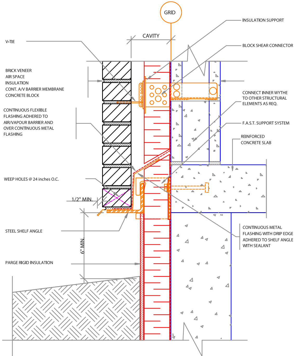
FIGURE 1 BRICK VENEER/CONCRETE BLOCK DETAIL AT FOUNDATION
